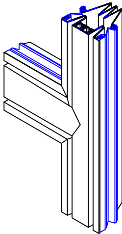
"T" MITER
